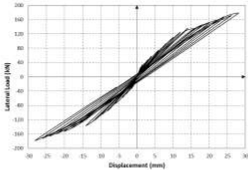
Fig 9.a. Hysteresis loops curves for model (S-01-FEM).
