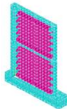
Fig. 7.e. Typical finite element meshing (solid walls).
