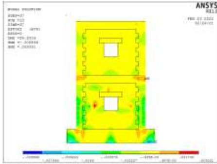
Fig 8.q. Mechanical strain at ultimate load (face with windows) - model at push case.
