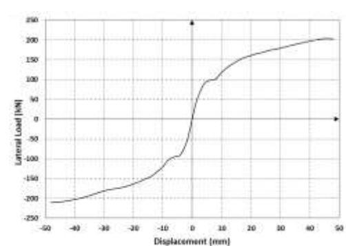
Fig 11.b. Envelope load-displacement curves for - model (S-02-FEM).
