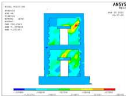
Fig 10.o. Mechanical strain at ultimate load (face with doors) – model (S-02-FEM) at push case
