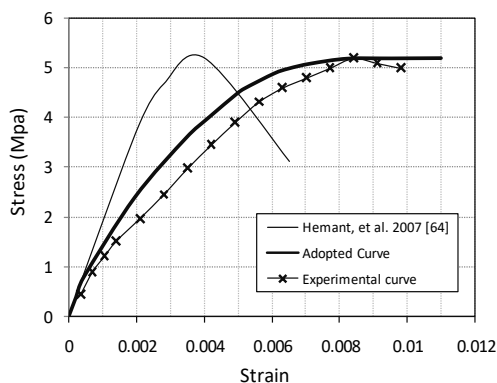
Fig. 5. Compressive stress-strain curves for masonry
