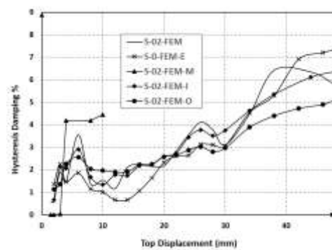
Fig 27.d. Hysteresis damping% for compared with model (S-02-FEM).
