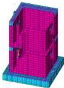
Fig 14. Finite element model characterization and meshing for model (S-01-FEM-M).
