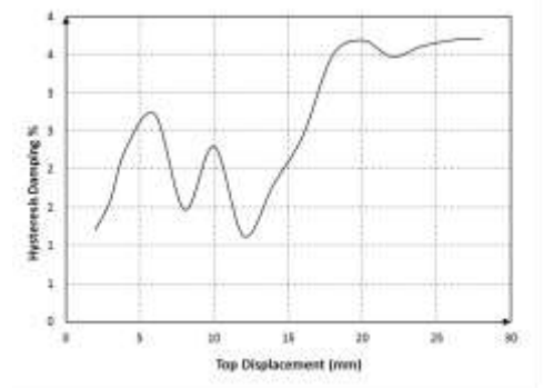
Fig 9.e Hysteresis Damping% for Model (S-01-FEM)
